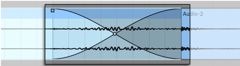
Crossfaded Clips.
